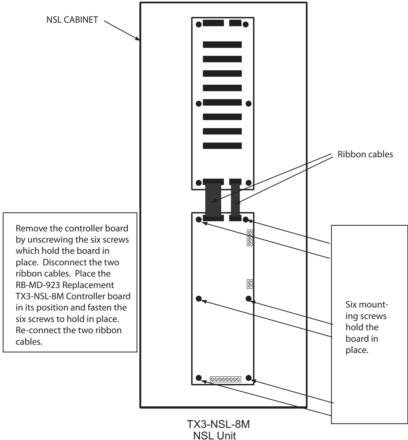
Figure 1: RB-MD-923 TX3-NSL-8M Board Replacement
